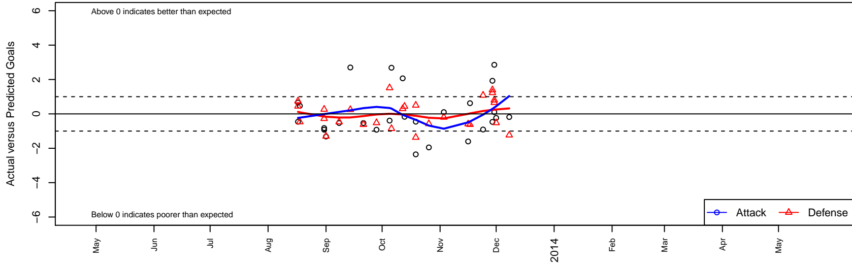
So Cal Blues Kale G01 Dots are actual minus expected GF (blue circles) and GA (red triangles). Blue line is smoothed change in attack strength. Red is smoothed change in defense strength.
